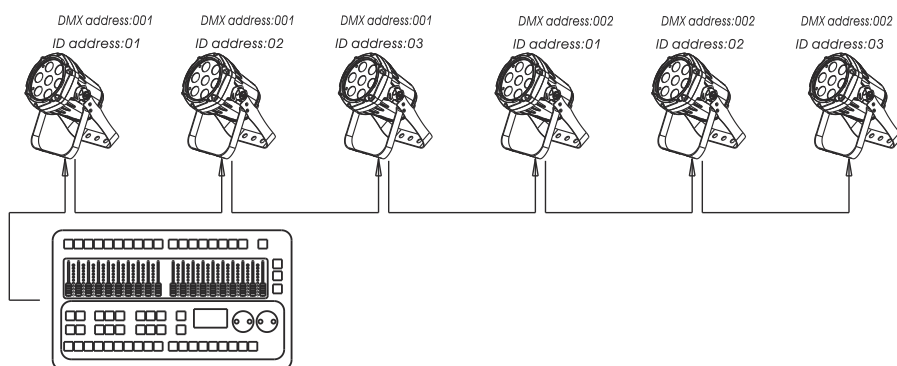
DMX 512 Controller
